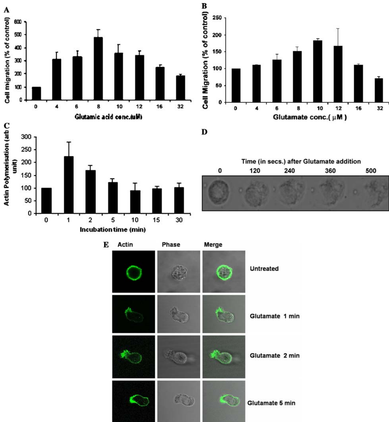
Fig. 3 Glutamate as the neutrophil migration factor. All data represents mean of three independent experiments. a Glutamate induces neutrophil migration (chemotaxis). The migration assay was performed either by using untreated cells ( 4 \times 10^5 cells/well) or with different doses of glutamate for 2 h. Glutamate was added to the lower chamber. b Glutamate induces neutrophil migration (chemokinesis). The migration assay was performed either by using untreated cells ( 4 \times 10^5 cells/well) or with different doses of glutamate for 2 h. Glutamate was added in equal concentration to both chambers. c Glutamate increases the synthesis of F-actin. Neutrophils were left untreated or treated with 8 \mu\text{M} of glutamate for specified time at 37^\circ\text{C} . Cells were fixed at the time points shown by addition of 10 vol of 4.6% paraformaldehyde in PBS. Treatment with carrier (water) did
